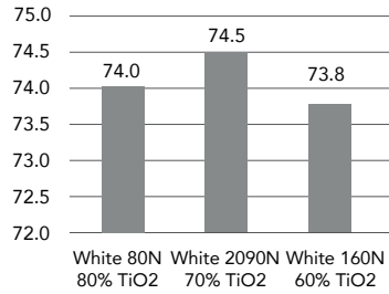
Whiteness of White Masterbatches containing different % of TiO 2
