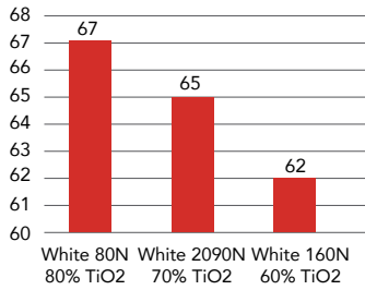
Opacity of White Masterbatches containing different % of TiO 2
